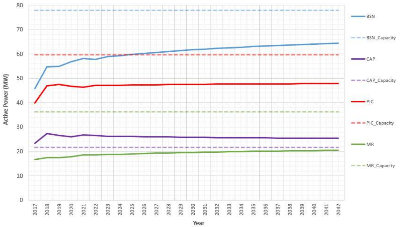
Figure 8: Picton South - 25 Year peak demand forecast - Substation (non-coincidental) PoE10%
