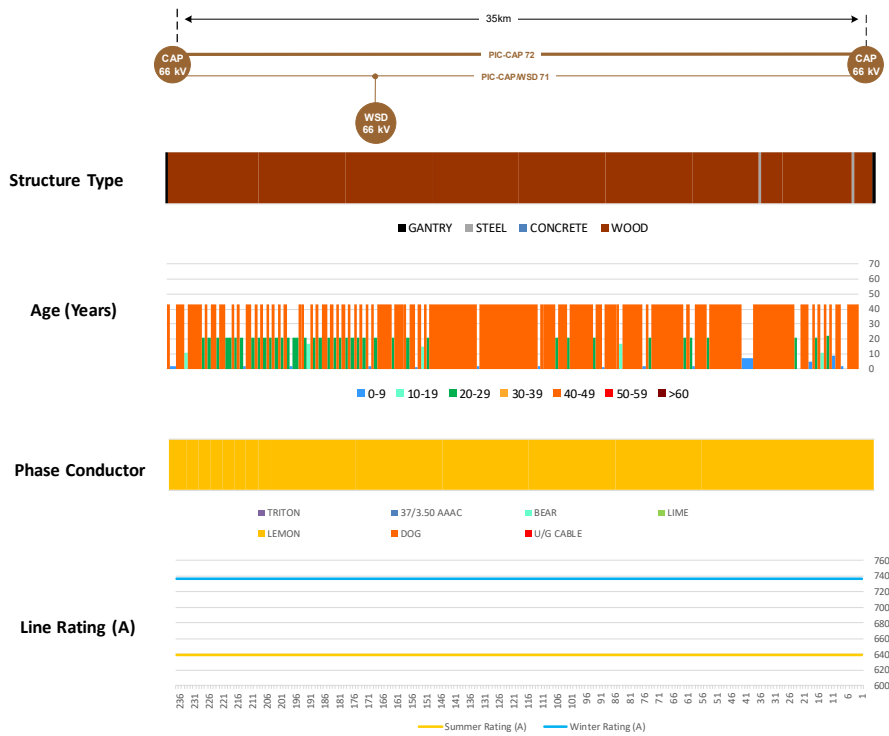
Figure 21: Picton-Capel/Westralian 71 transmission line asset information
