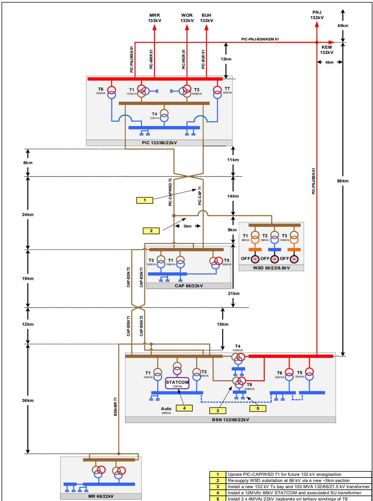
Figure 29: Picton South Network – Completion of Stage 1 works
