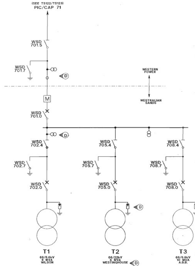
Figure 31: Westralian Sands SLD
