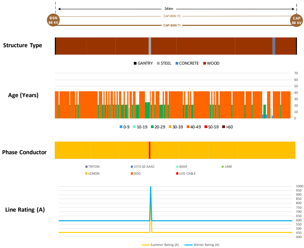
Figure 23: Capel-Busselton 71 transmission line asset information
