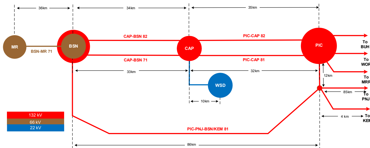
Figure 6: Picton South Network Development – Long term strategic view
